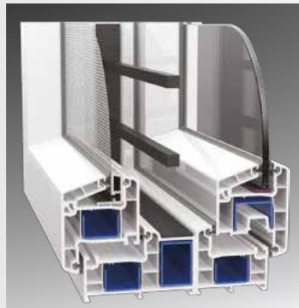
Casement Window with Grill & Mesh
