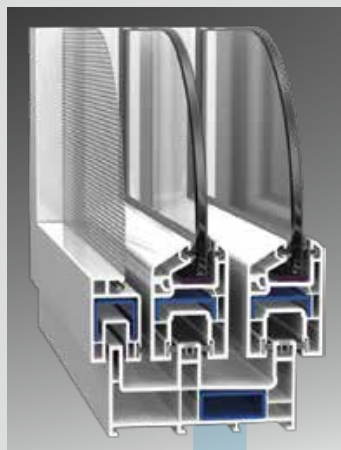
2.5 Track 2 Panel with Screen
