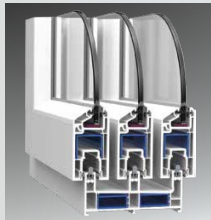
3 Track 3 Panel
